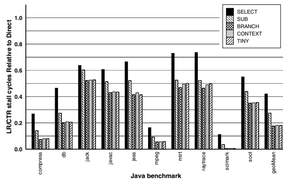
(b) PPC7410 lr/ctr stalls
